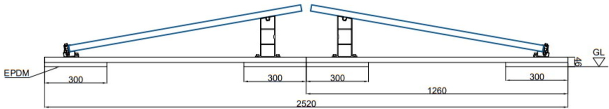
Side view (east-west orientation)
